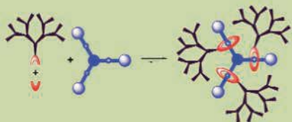
A representation of the synthesis process and the generation 1 dendrimer.
